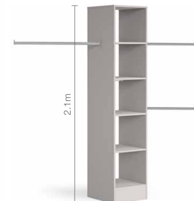
TOWER UNITS Available in two widths of 450mm and 600mm with a choice of a 3 drawer combination or shelves only. All drawers come with soft close as standard. Maximum opening width 2800mm x Tower Unit height 2100mm x Depth 500mm.
